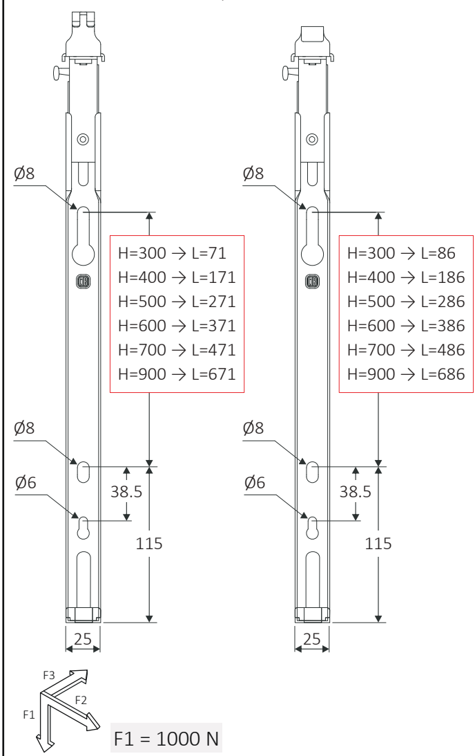
F7LG 10-11 with grille
