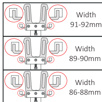
Assembly instructions
